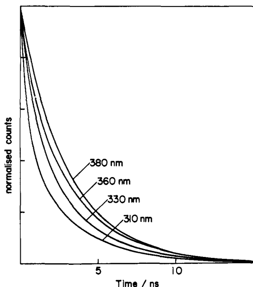
Figure 2. Normalized calculated "best fit" emission decay profiles after deconvolution of the corrected emission decay profiles of aqueous tryptophan. \lambda_{\text{ex}} 280 nm. \lambda_{\text{em}} (a) 310, (b) 330, (c) 360, (d) 380 nm. Curves (a), (b), and (c) are the calculated decay profiles for two exponential decay components. Curve (d) is for one exponential decay component.
